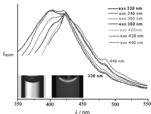
Figure 1. The luminescence emission spectra of HPAA12, the inset image (A) is the optical micrograph of HPAA12 solution without filter, and (B) is its optical micrograph with filter.
